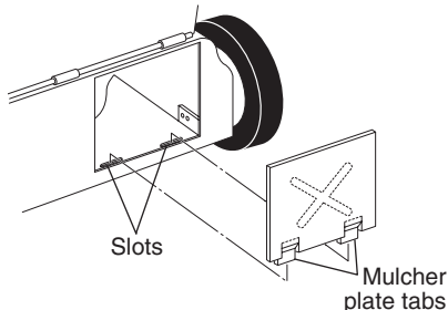
MULCHER "PLUG"
