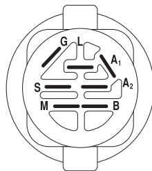
IGNITION SWITCH
