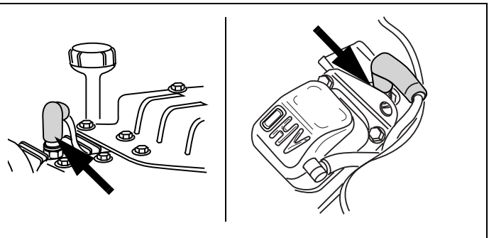
Figure 4. Typical Spark Plug Connection
