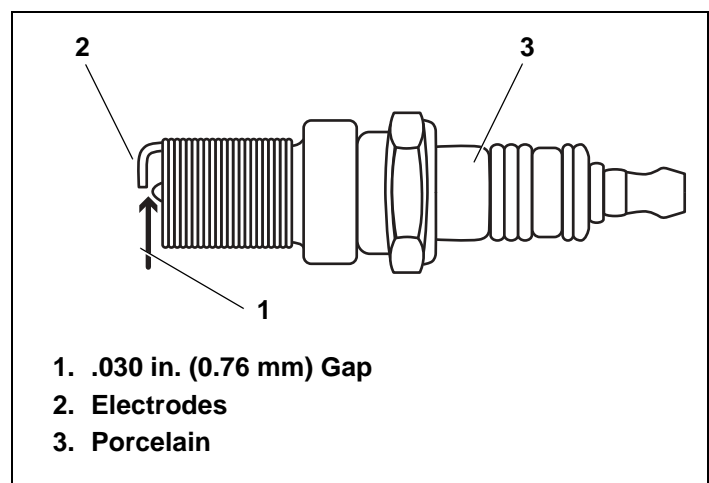
Figure 23. Spark Plug
