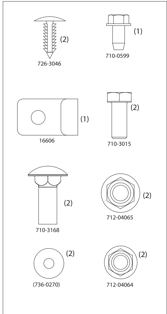
Hardware Pack 689-00094
