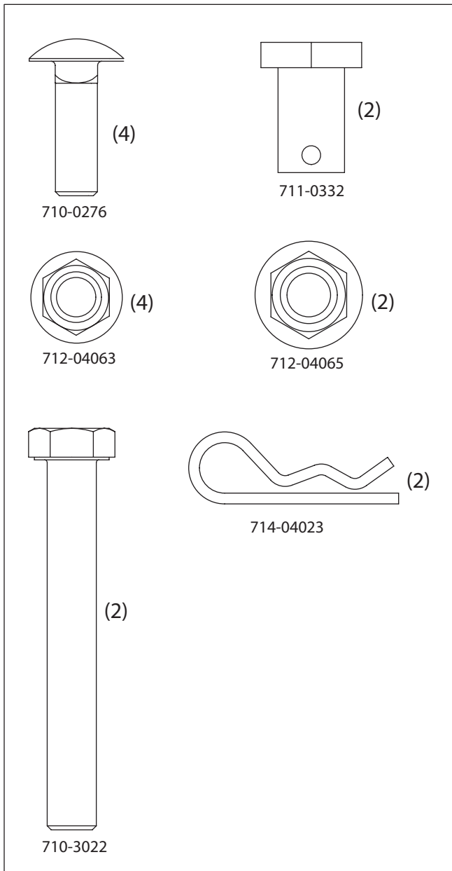
Hardware Pack 689-00093
