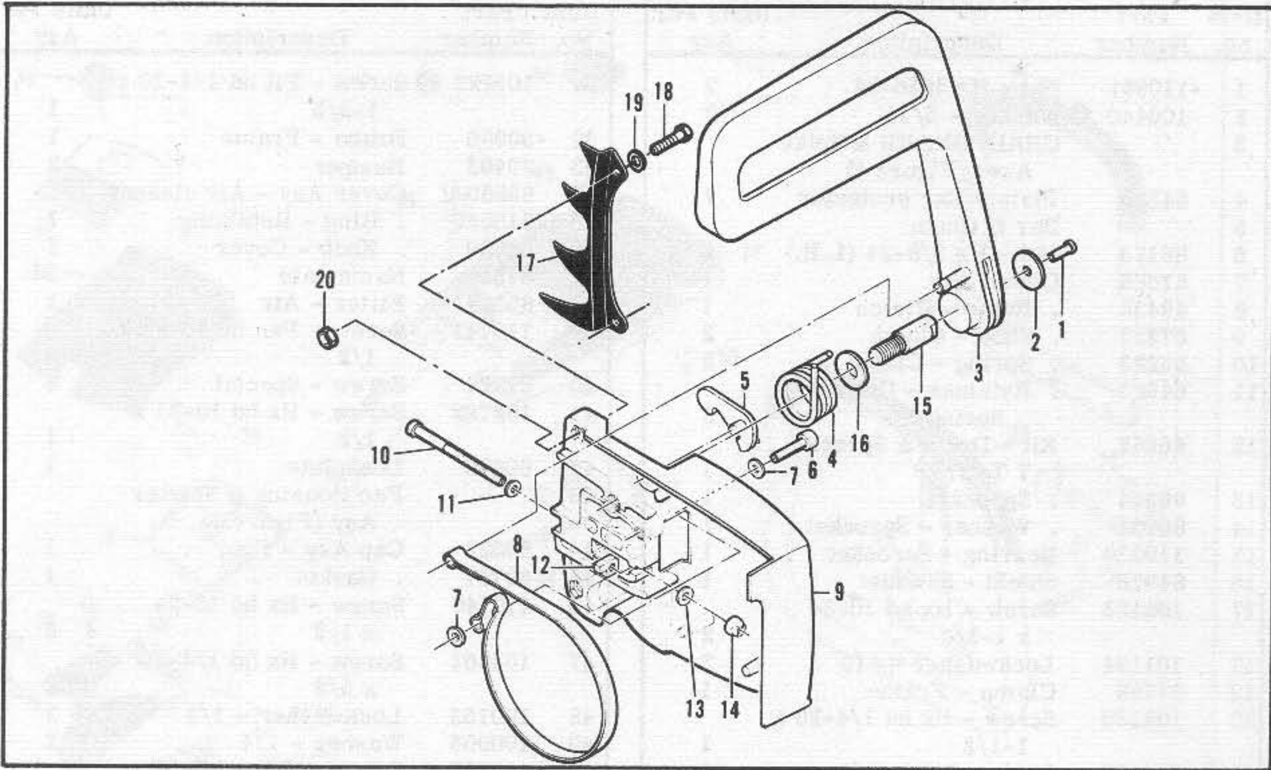
Figure 2. CHAIN BRAKE and Spike Assemblies.
