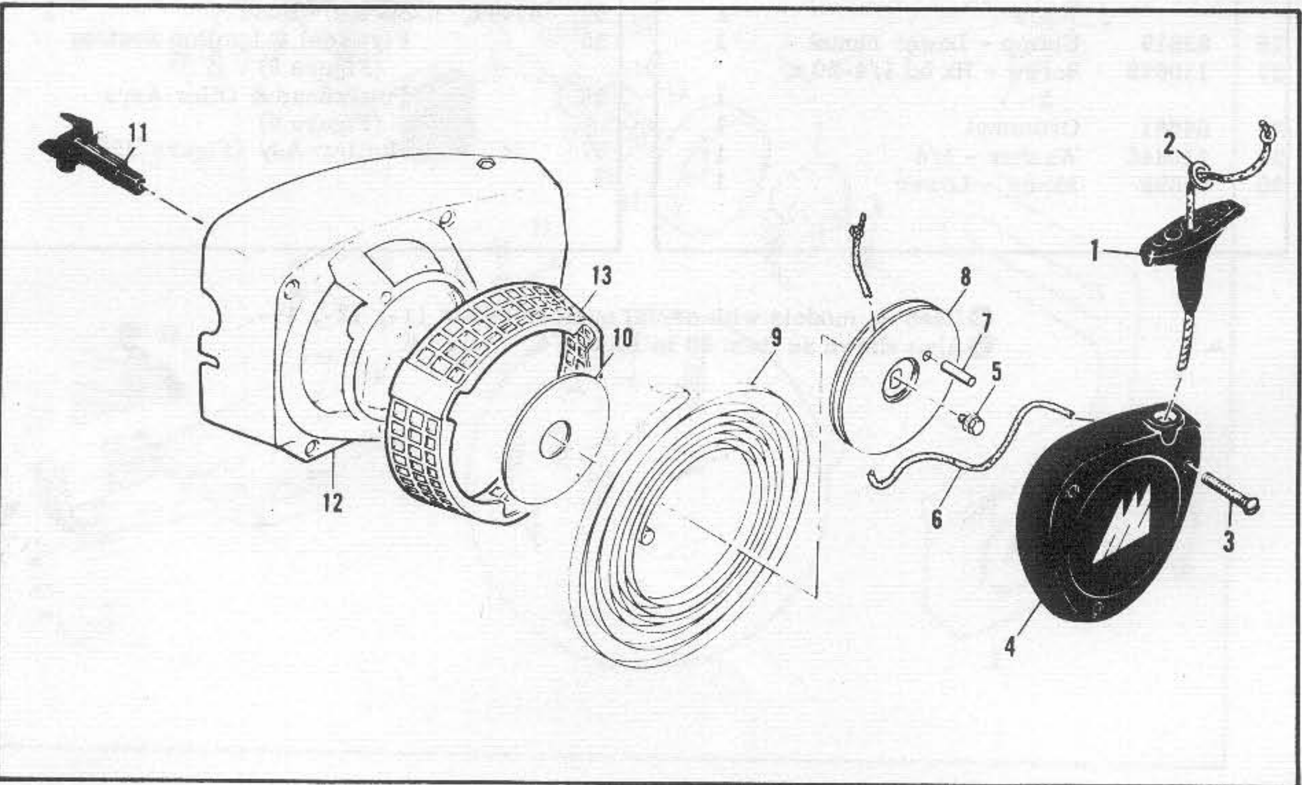
Figure 3. Fan Housing & Starter Assemblies.
