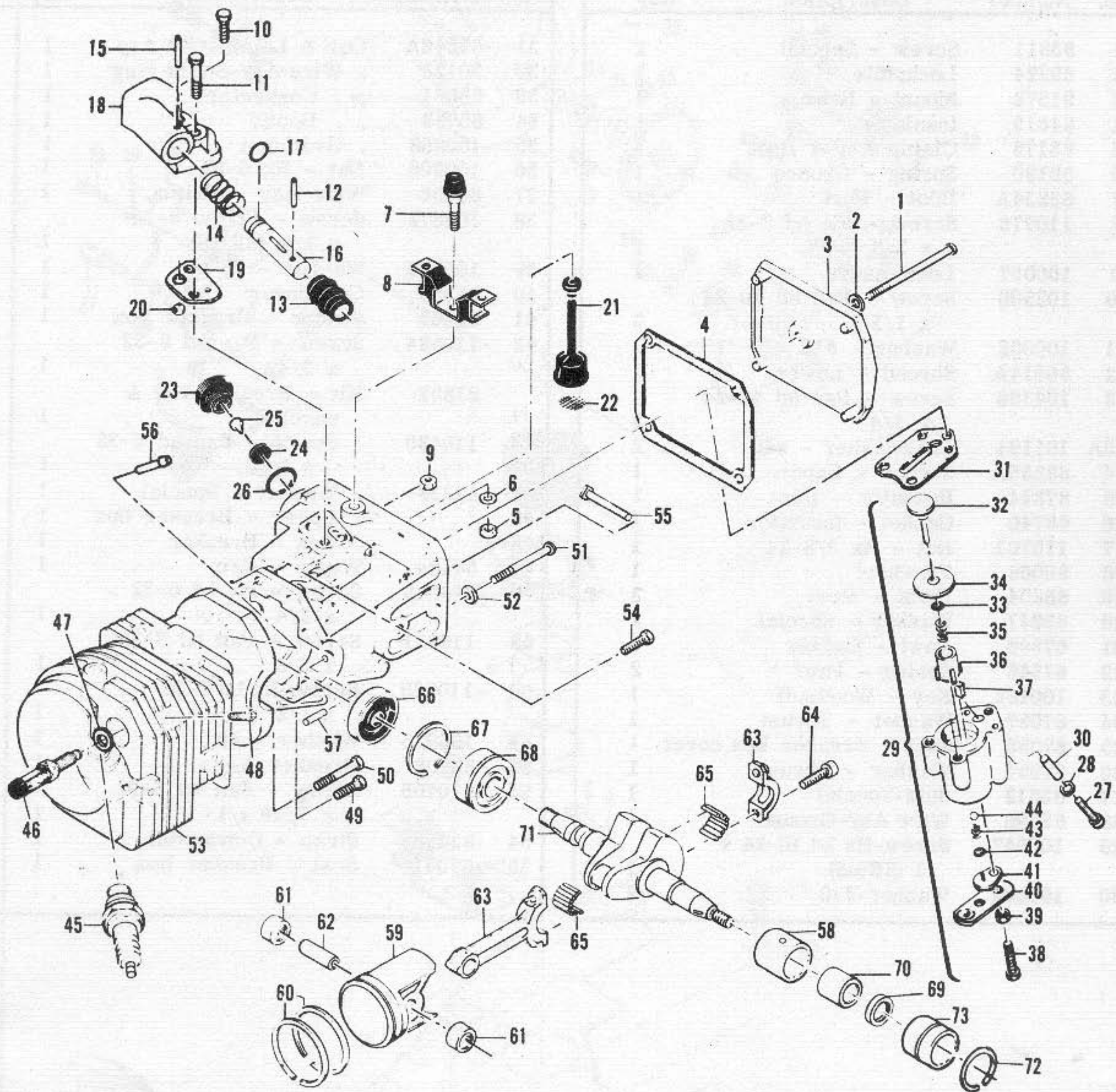
Figure 9. Powerhead & Oiler Assemblies.
