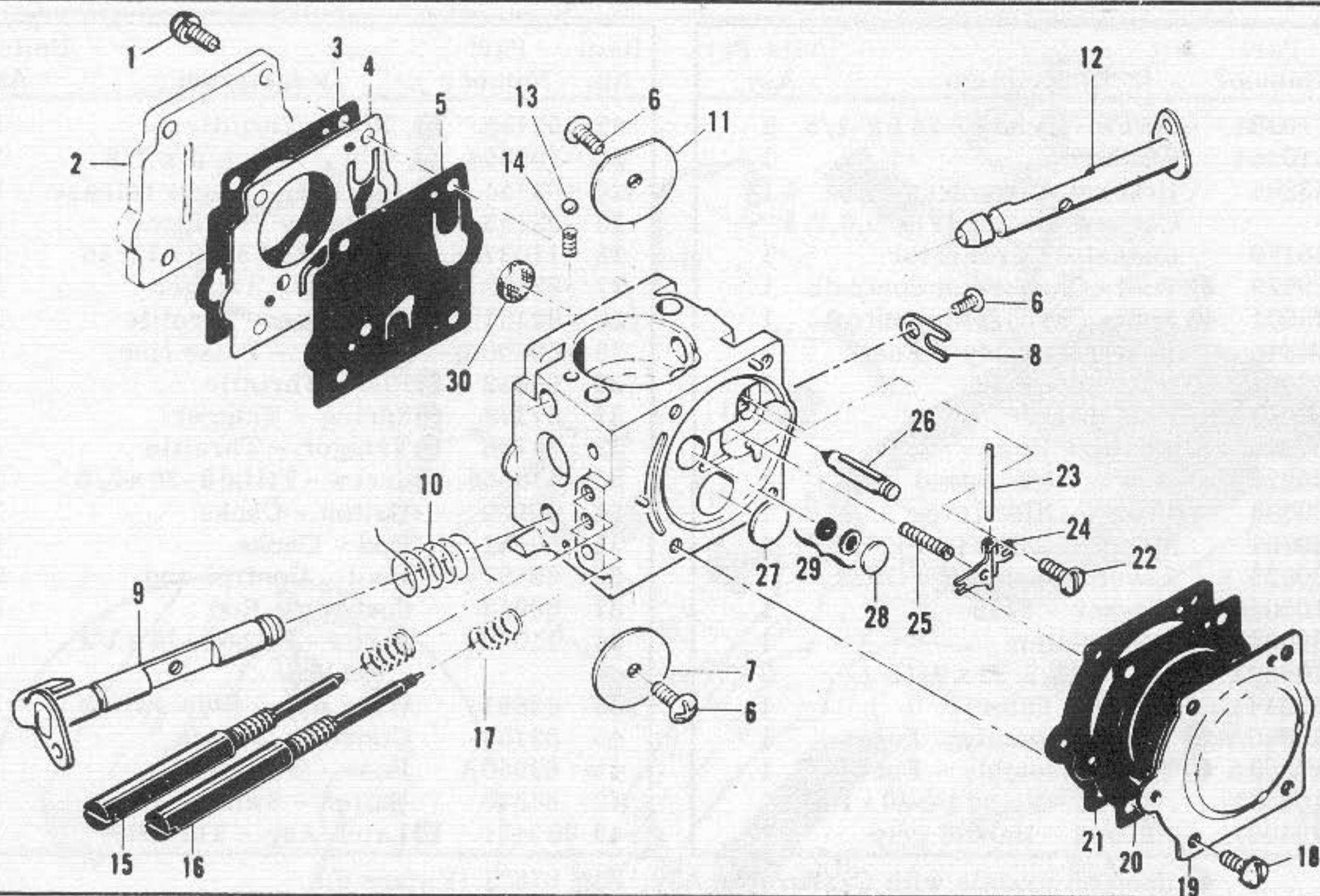
Figure 6. Carburetor.
