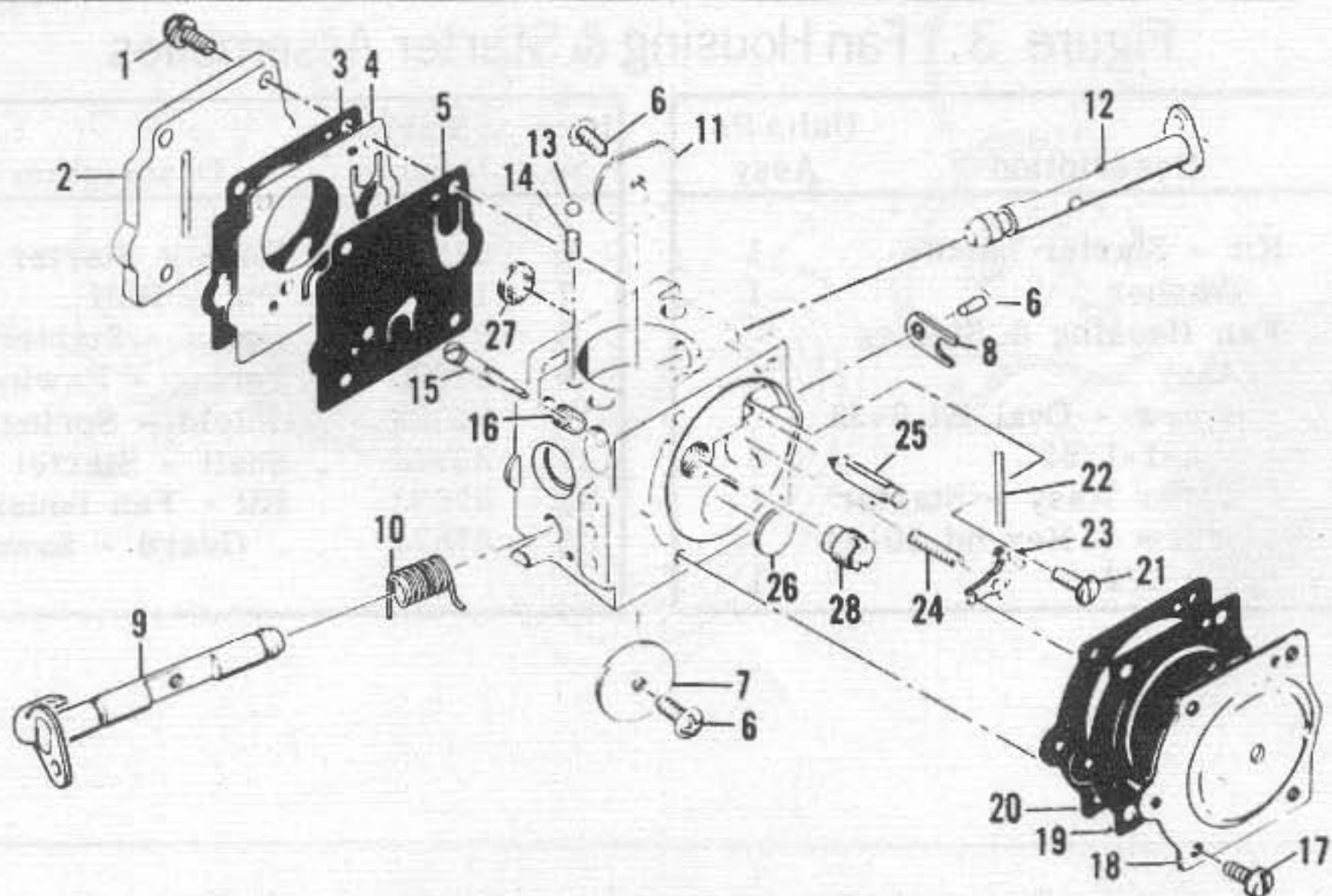
Figure 5. Carburetor Assembly.
